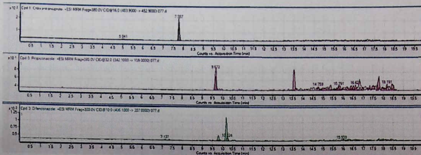
Figure 4.1: Example of MRM chromatogram obtained from one of the personal air samples of the respondent
