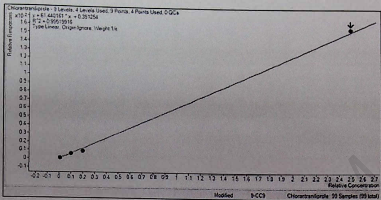
Figure 3.2: Calibration curve of chlorantraniliprole
