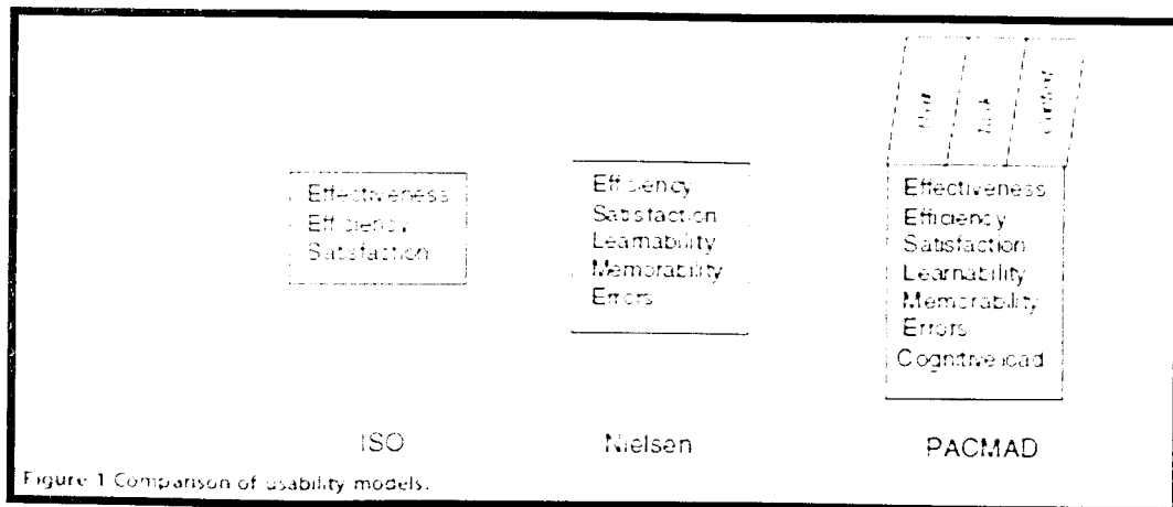
Figure 2.1: Usability Model
